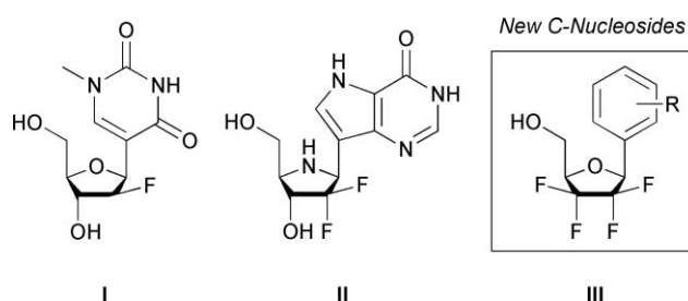
Fig. 1 Monofluoro-, difluoro- and tetrafluoro- C -nucleosides.
