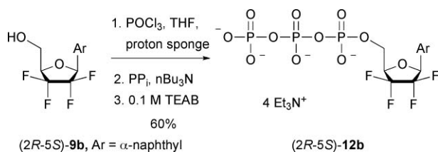
Scheme 2 Triphosphorylation of (2 R ,5 S )- 9b .
