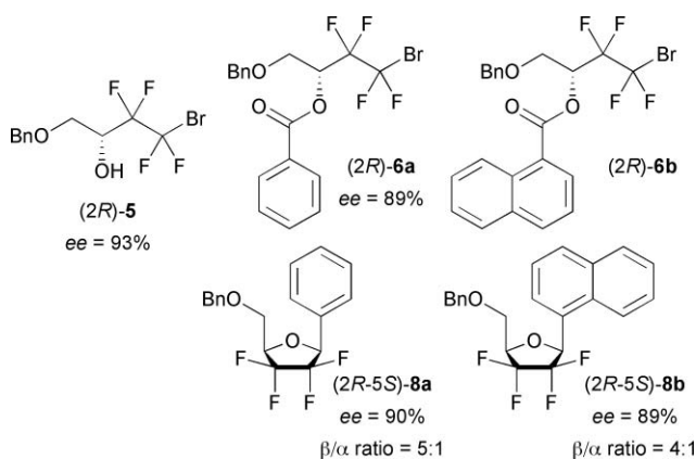
Fig. 3 Asymmetric synthesis of 8a and 8b .
